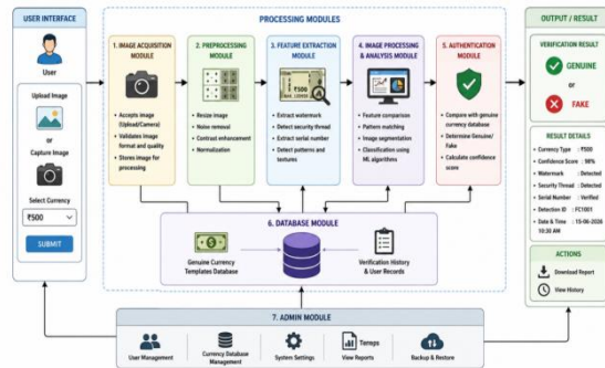
FAKE CURRENCY DETECTION USING IMAGE PROCESSING SYSTEM ARCHITECTURE
